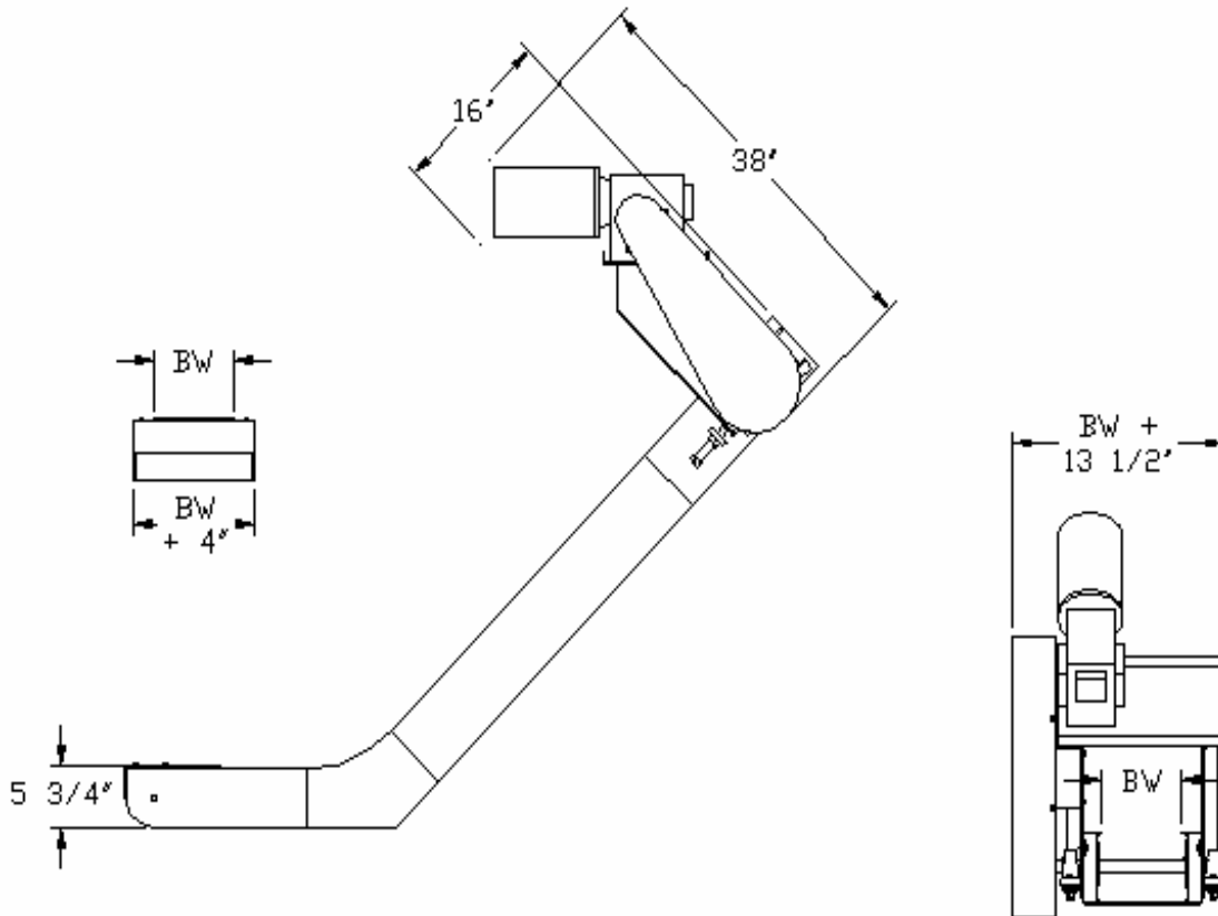
45° TOP MOUNT DRIVE
